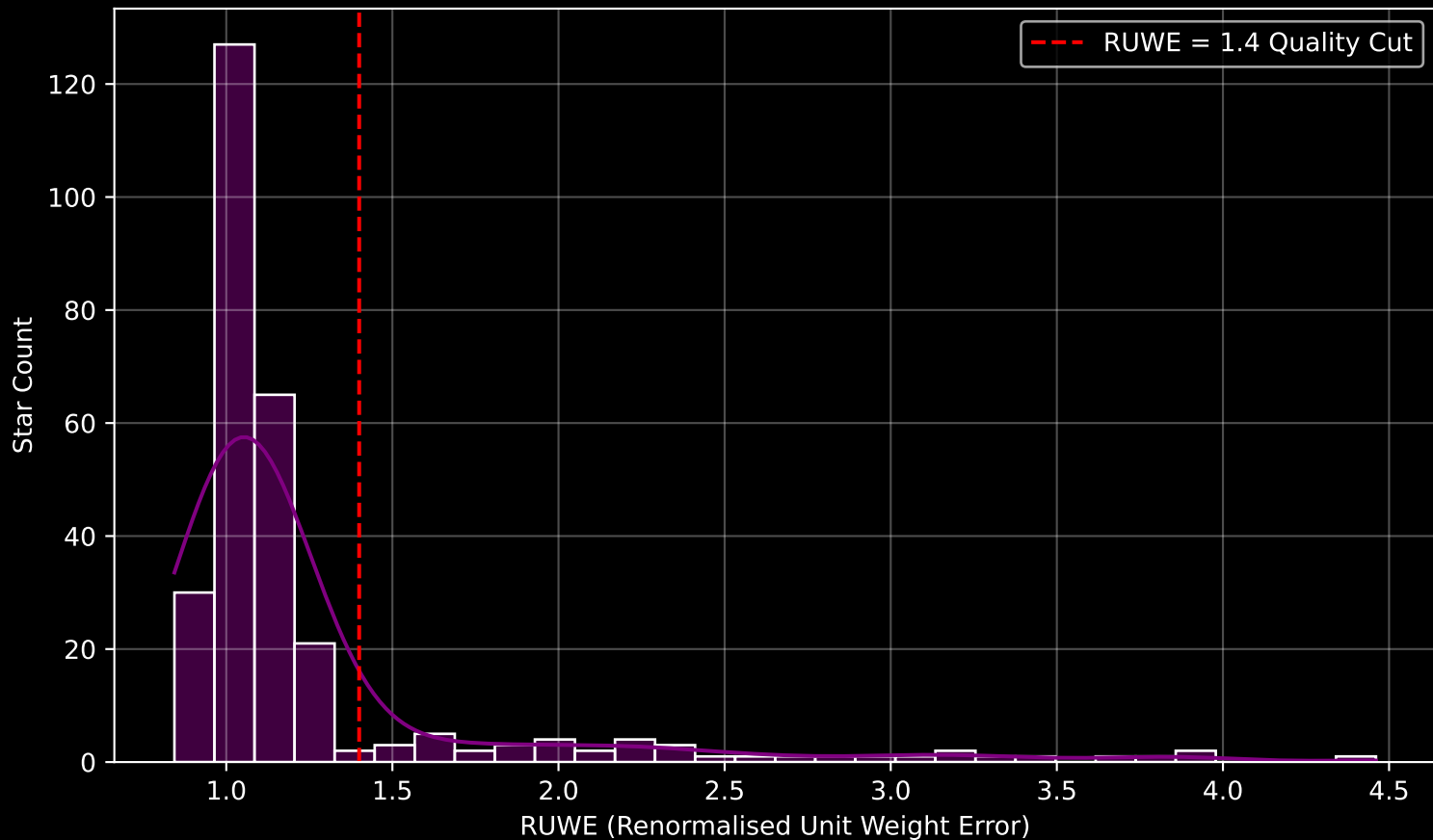
GALAH DR4 Field [212] RUWE Distribution (n= 286)
