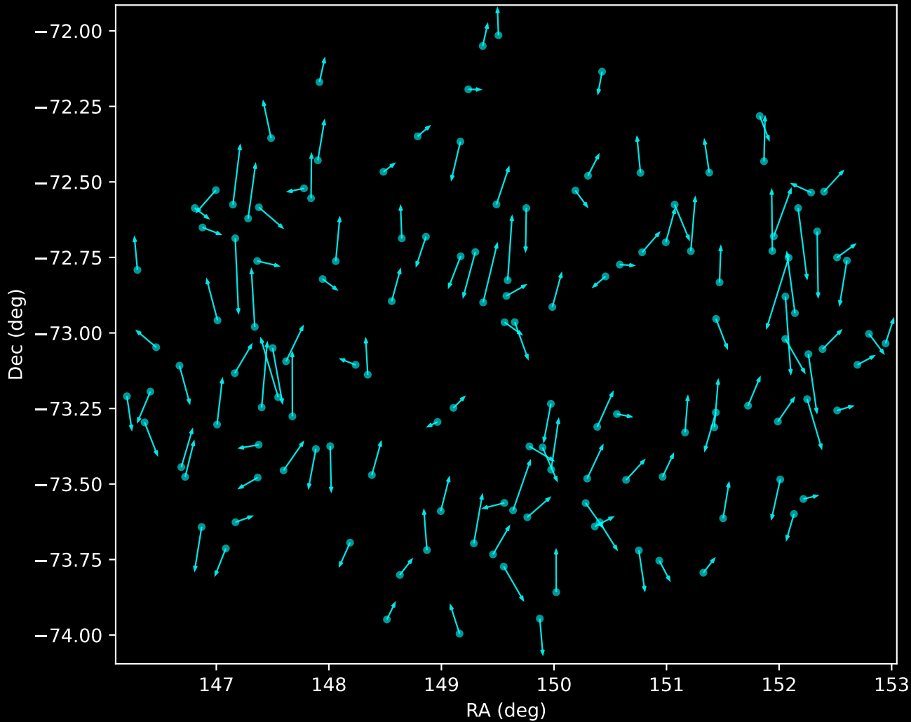
GALAH DR4 Noise Stream Proper Motion Vectors (n=136)
