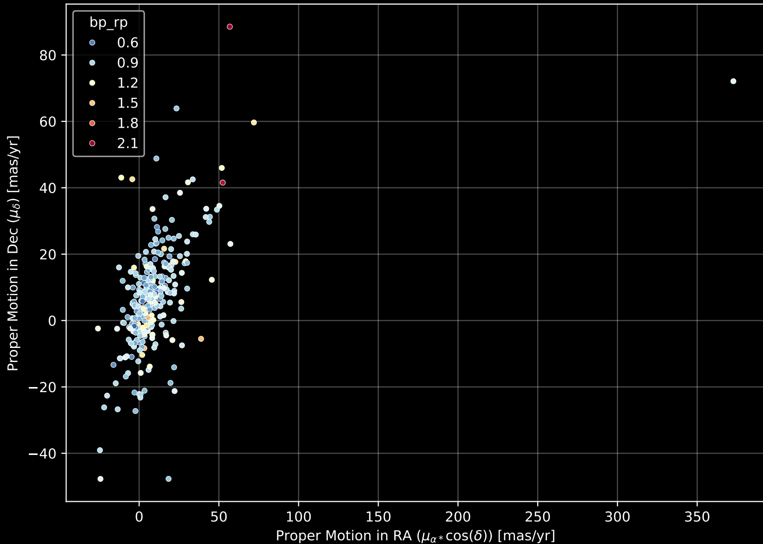
GALAH DR4 Field: [212] Proper Motion Diagram (n= 298)
