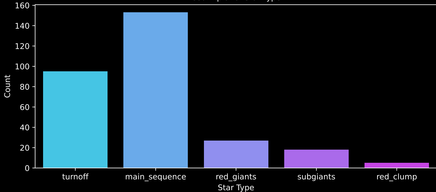
GALAH DR4 Field: [212] Count plot of Star Type
