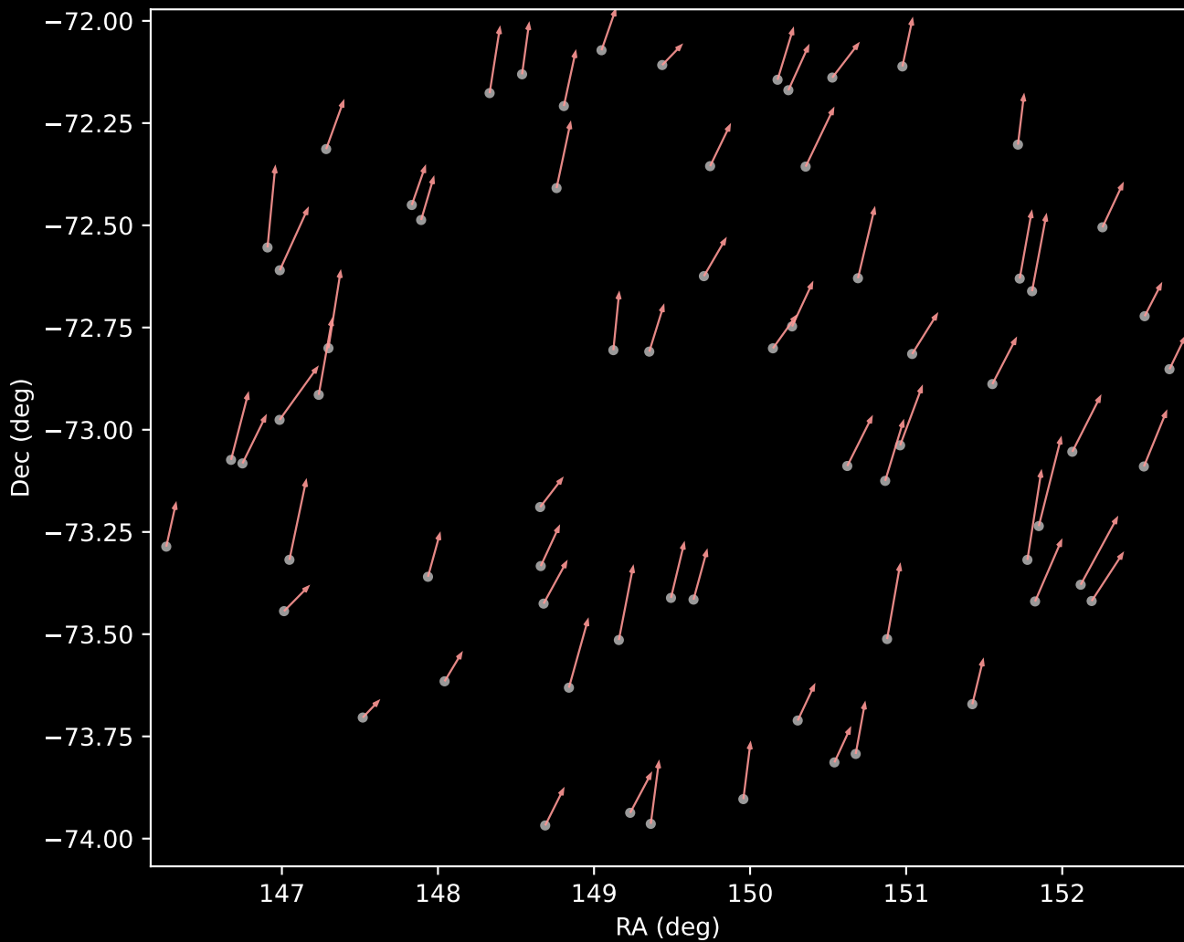
GALAH DR4 Cluster 7 Proper Motion Vectors (n=68)
